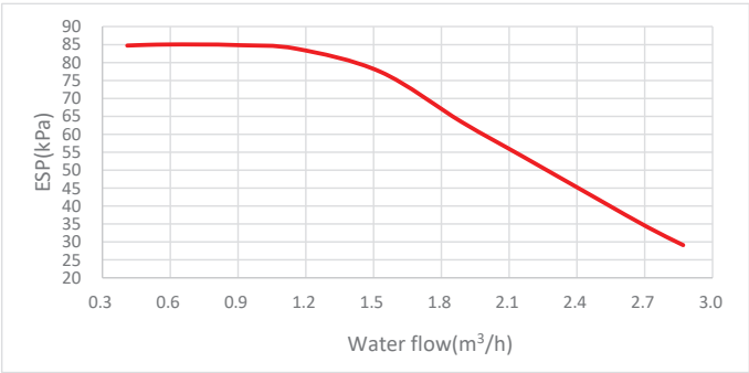
Figure 2-6.1: HPM-14(22,28,34)CH40(65,84,100)AERIs R32-1 hydronic performance 1
