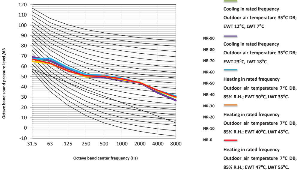
Figure 2-7.7: HPM-48CH140AERIs R32-3(3H9) octave band levels
