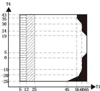
Figure 2-5.3: Domestic hot water operating limits 1
