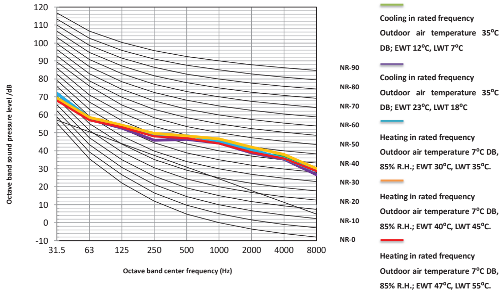
Figure 2-7.5: HPM-34CH100AERIs R32-1(1H3) octave band levels
