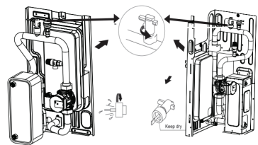
Figure 3-3.2: Water flow switch
