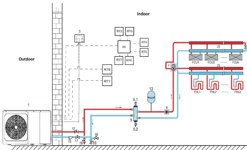
Figure 1-5.3: Application 2- Mode set control
