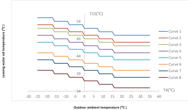
Figure 3-9.3: High temperature curves for heating mode 1
