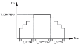
Figure 3-7.45: FLOOR DRYING UP settings
