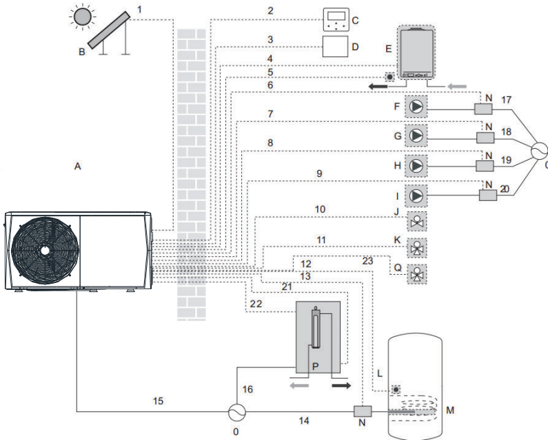
Figure 3-4.4: Wiring overview for 8/10/12/14/16kW models
