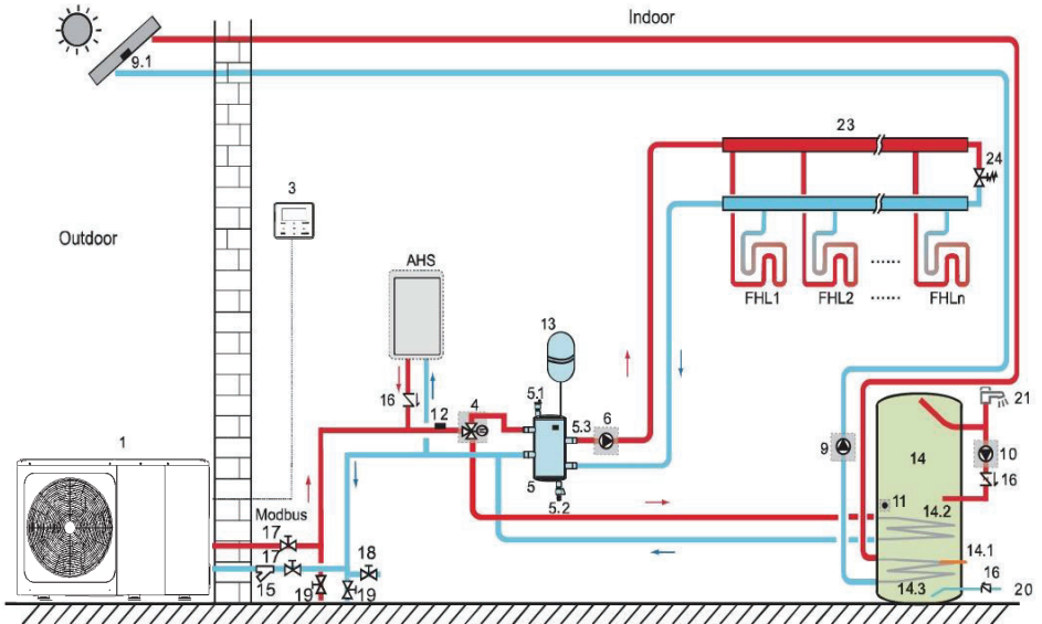
Figure 1-5.1: Application 1
