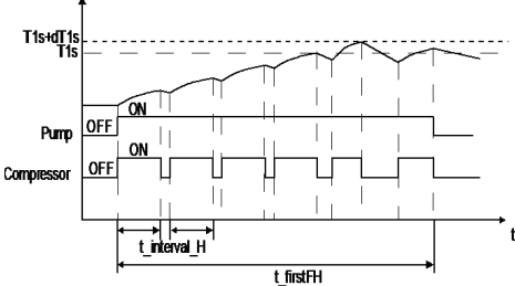
Figure 3-7.42: Preheating for floor
