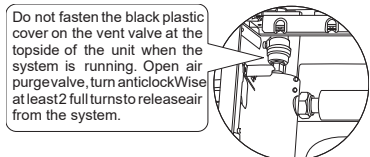
Figure 3-3.3: Air purge valve
