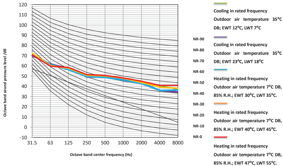
Figure 2-7.9: HPM-41CH120AERIs R32-3(3H9) octave band levels
