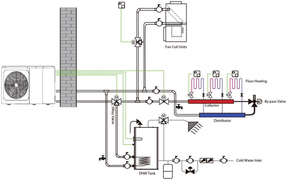
Figure 1-1.1: System schematic
