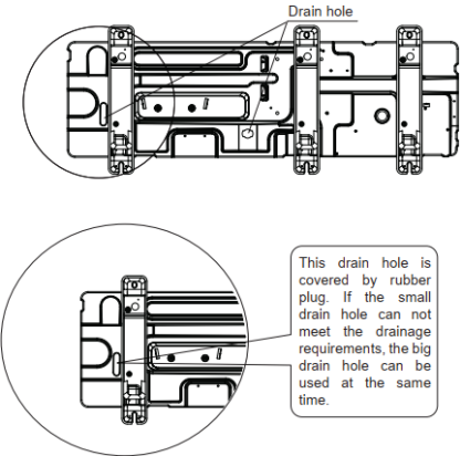
Figure 3-2.7: 8/10/12/14/16kW models drainage hole
