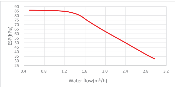
Figure 2-6.2: HPM 41(48,53)CH120(140,155)AERIs R32-3 performance 1
