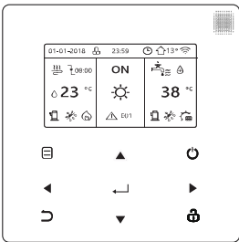
Figure 3-7.1: User interface
