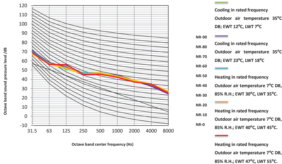
Figure 2-7.5: HPM-34CH100AERIs R32-1(1H3) octave band levels
