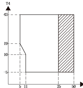
Figure 2-5.2: Cooling operating limits
