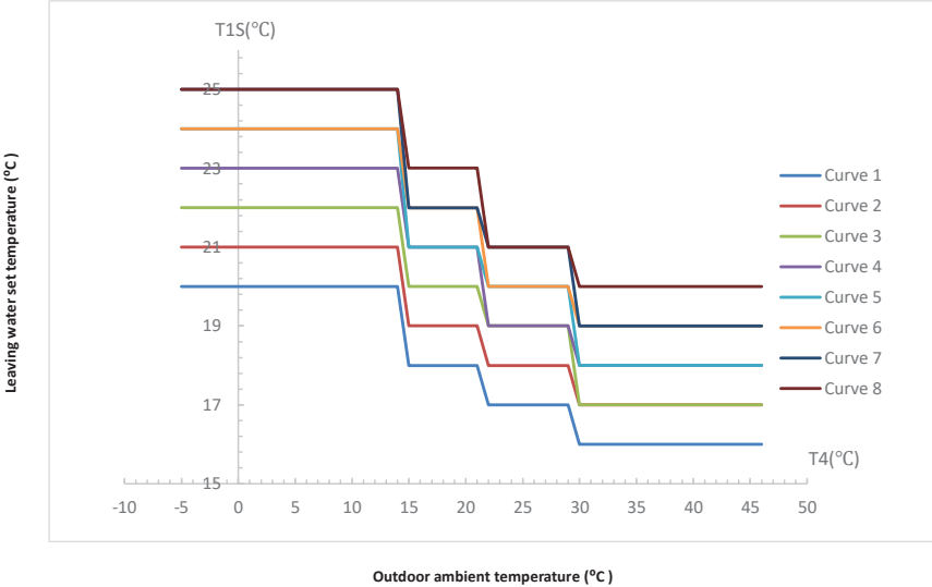
Figure 3-9.5: High temperature curves for cooling mode 1
