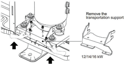
Figure 3-2.12: Remove the transportation support
