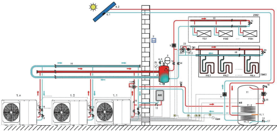
Figure 1-5.5: Application 3- Parallel system control
