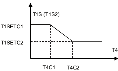
Figure 3-9.7: Automatic setting curve for cooling mode
