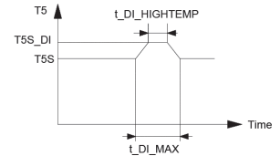
Figure 3-7.8: DHW tank disinfection
