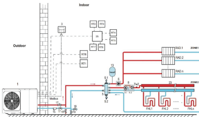
Figure 1-5.4: Application 2-Double zone control
