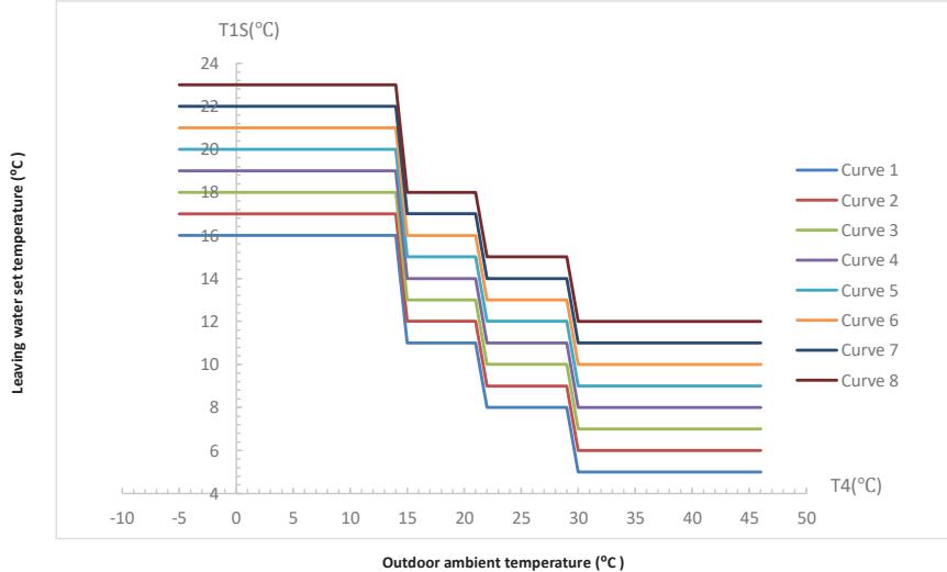
Figure 3-9.4: Low temperature curves for cooling mode 1
