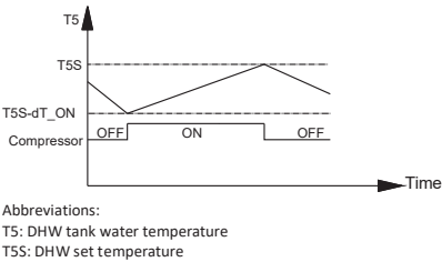
Figure 3-7.5: dT5_ON
