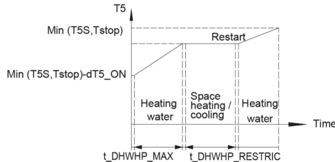
Figure 3-7.9: Operation in DHW PRIORITY
