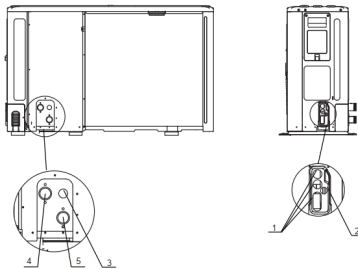
Figure 3-4.2: Wiring hole for 8~16kW models
