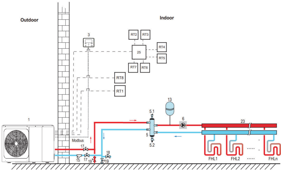
Figure 1-5.2: Application 2-One zone control
