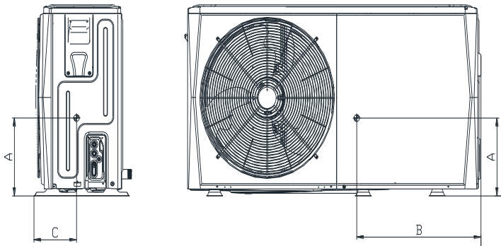
Figure 2-3.1: HPM-14(22)CH40(65)AERIs R32-1 / HPM-14(22)CH40(65)AERIs R32-1H3 dimensions and center of gravity (unit: mm)
