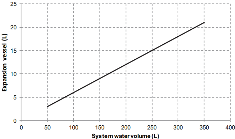
Figure 3-3.1: Expansion vessel volume
