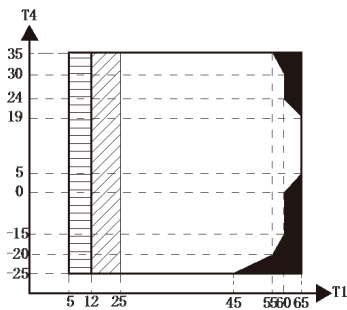
Figure 2-5.1: Heating operating limits 1
