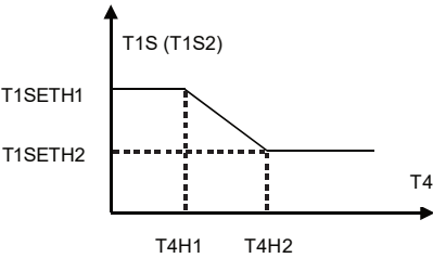
Figure 3-9.6: Automatic setting curve for heating mode
