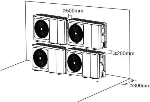
Figure 3-2.11: Multi-row installation
