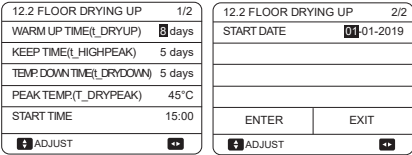
Figure 3-7.44: FLOOR DRYING UP menu
