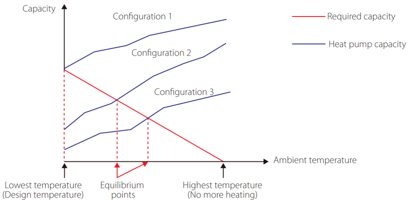
Figure 1-1.2: System configurations
