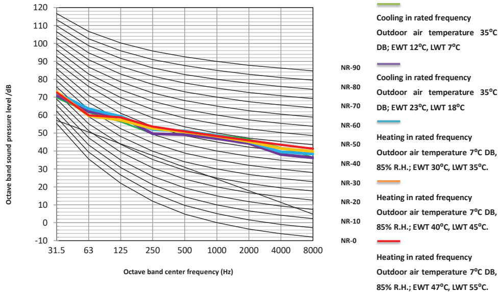
Figure 2-7.11: HPM-53CH155AERIs R32-3(3H9) octave band levels
