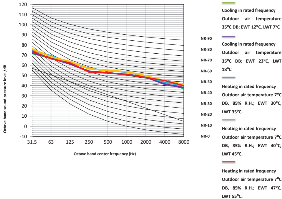
Figure 2-7.11: HPM-53CH155AERIs R32-3(3H9) octave band levels
