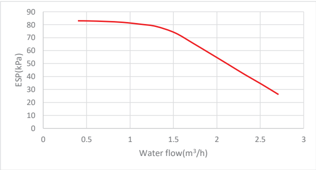
Figure 2-6.3: MHC-V4(6, 8, 10)W/D2N8-BE30 / MHC-V8(10)W/D2N8-BE90hydraulic performance 1
