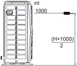
Figure 2-6.1: Sound pressure level measurement (unit: mm)
