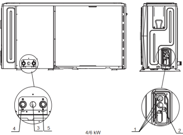
Figure 3-4.1: Wiring hole for 4/6kW models
