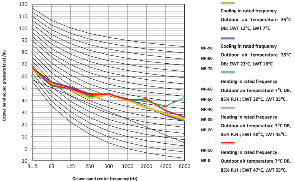
Figure 2-7.3: HPM-22CH65AERIs R32-1(1H3) octave band levels
