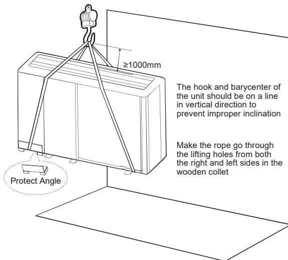
Figure 3-2.1: Hoisting the unit
