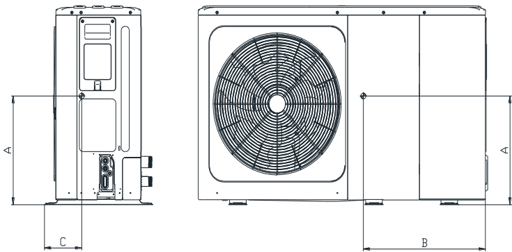
Figure 2-3.2: HPM-28(34)CH84(100)AERIs R32-1(1H3)/HPM-41(48,53)CH120(140,155)AERIs R32-3(3H9) dimensions and center of gravity (unit: mm)
