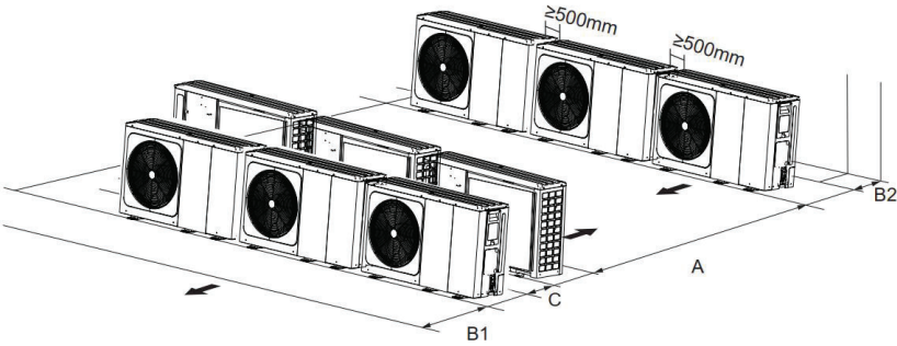
Figure 3-2.11: Multi-row installation
