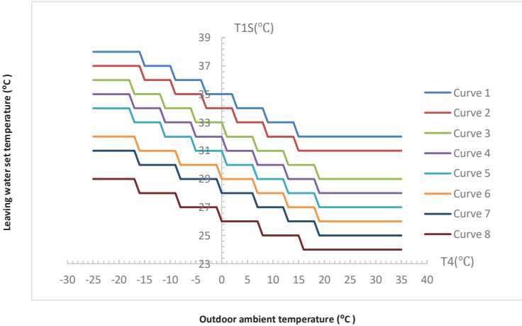
Figure 3-9.2: Low temperature curves for heating mode 1
