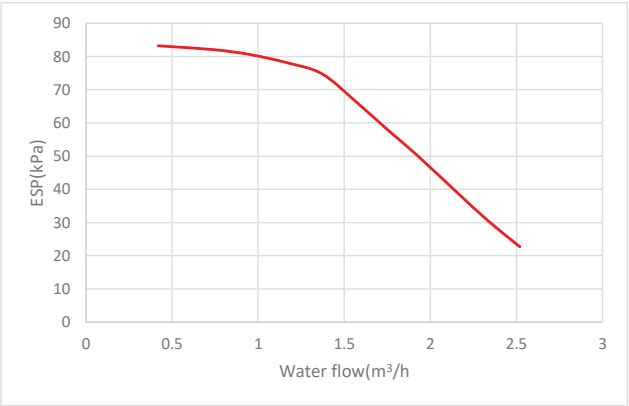
Figure 2-6.4: HPM-41(48,53)CH120(140,155)AERIs R32-3H9 hydraulic performance 1
